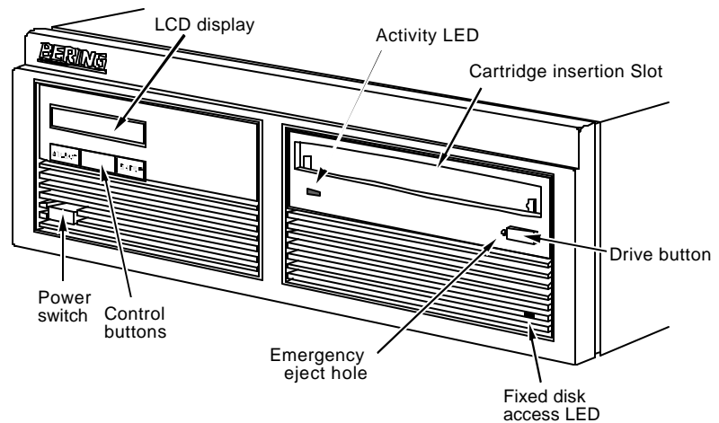
Figure 3-1: OptiPac 2652MD front panel
