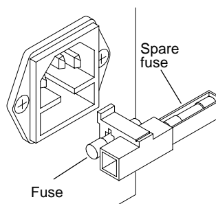
Figure 6-1: Replacing the AC fuse
