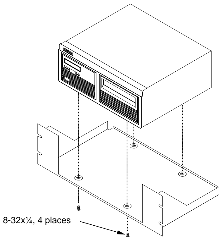
Figure B-1: Attaching the OptiPac to the rack mount
