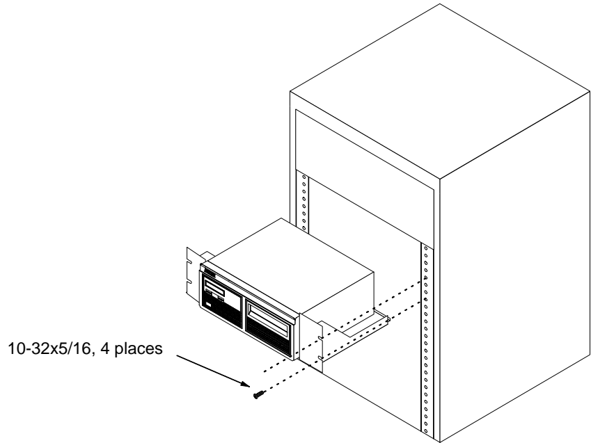
Figure B-2: Installing the rack mount into a chassis
